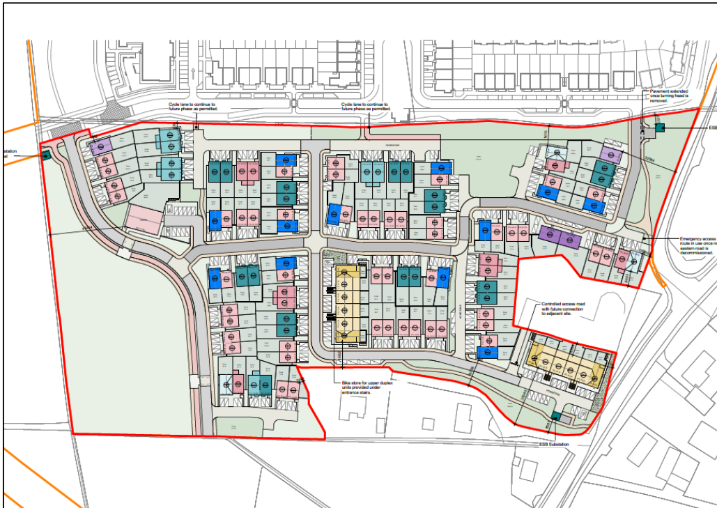
Figure 3.1: Proposed Site Layout Plan (Source: Howells Architects)
