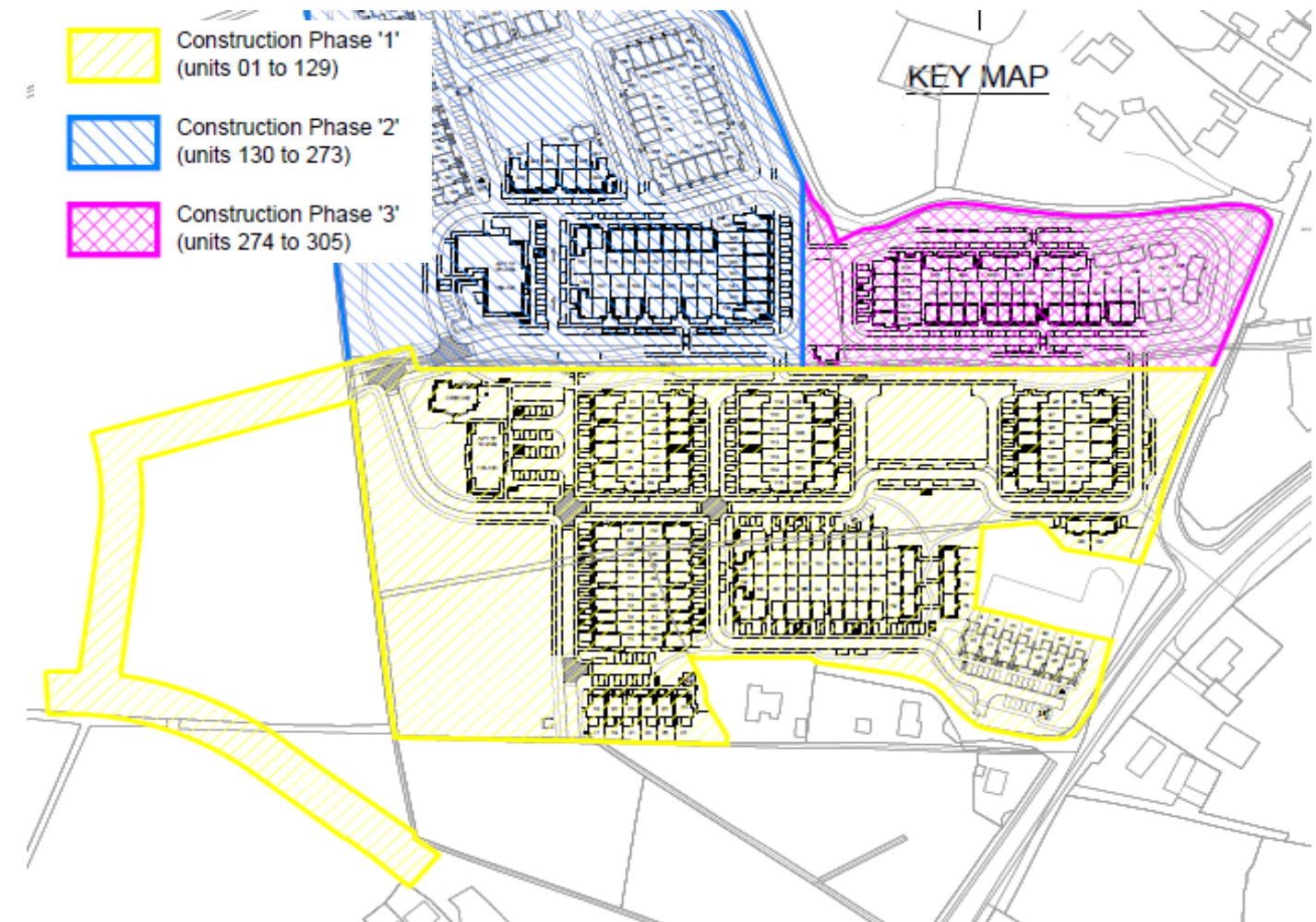
Consented phasing
